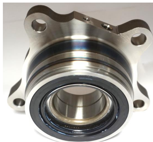
44BWK02R-Y-2CA17**01
